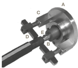
A: Tooling holder complete B: Mandrel for internal skiving C: Holder for external skiving knife D: External skiving knife E: Internal skiving knife
