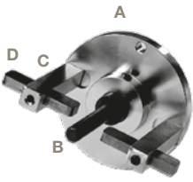
A: External skiving tool holder B: Mandrel for external skiving C: Holder for skiving tool D: External skiving knife
