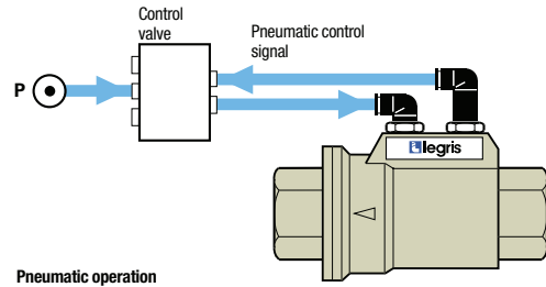
Pneumatic operation
