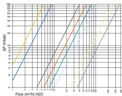
Pressure Drop
